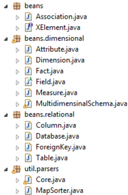
Figure 14. X-ETLproject architecture
